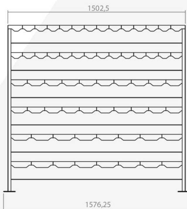
Vista Frontal
